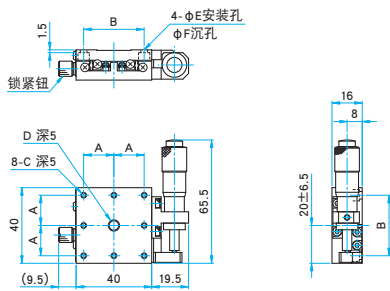
TSD-401SZ/401SZUU
