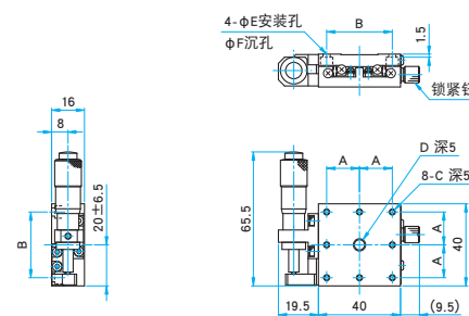
TSD-401SRZ/401SRZUU
